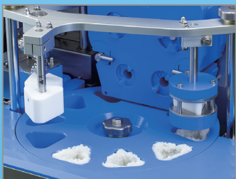
Fill Rice and Make Hole
